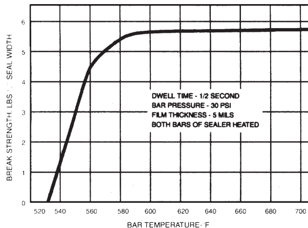
Figure 1. Effect of Bar Temperature Upon Seal Strength of DuPont FEP Film Pressure
