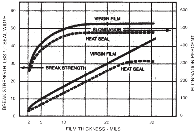
Figure 6. Heat Seal Strength and Elongation Obtainable with DuPont FEP Film Compared to Virgin Film
