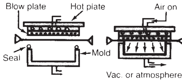
PRESSURE FORMING - FEMALE MOLD
