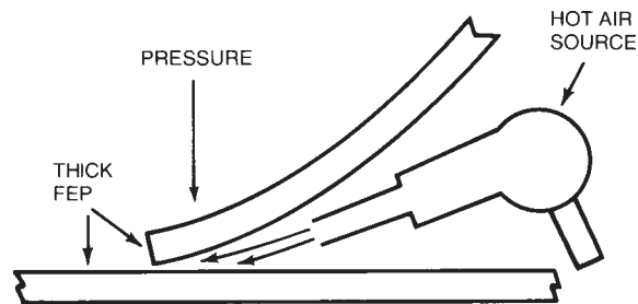
Illustration A. Hot Air Sealing of Thick Films
