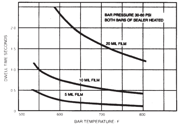
Figure 5. Temperature-Time Relationship for Obtaining Fusion Heat Seal with DuPont FEP Film
