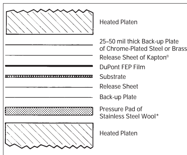
Figure 8. Platen Press Laminating
