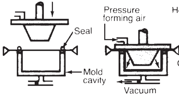
PRESSURE FORMING w PLUG ASSIST FEMALE MOLD
