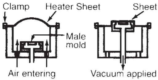
BLOWBACK FORMING WITH PRESSURE
