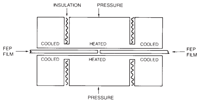
Illustration C. Transparent Butt Seal
