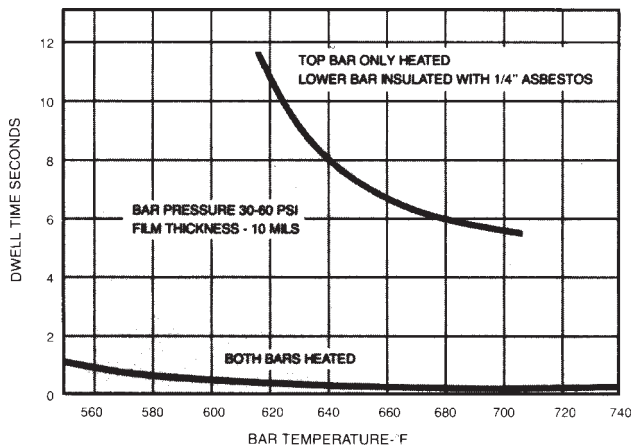
Figure 3. Effect of Bar Heating Upon Temperature-Time Relationship for Heat Sealing DuPont FEP Film
